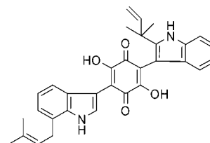
Demethylasterriquinone B1
